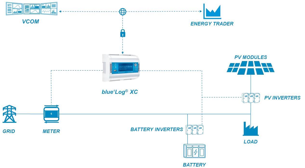
Example of a Hybrid EMS system layout
